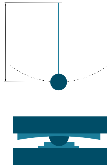
The principle of the Sliding Pendulum Isolator
